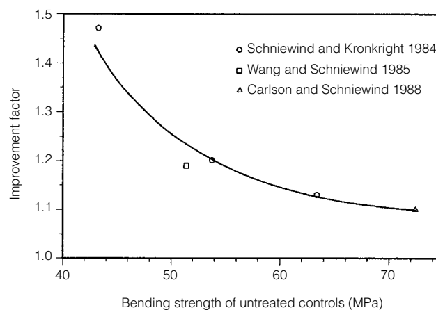
Figure 1 Improvement factor: ratio of bending-strength values of wood treated with Butvar B98 to bending-strength values of untreated wood, for deteriorated Douglas-fir at various levels of residual bending strength (degrees of deterioration).
