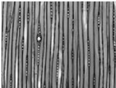
Figure 8 Tangential section of spruce ( Picea sp.) showing several uniseriate rays and one fusiform ray with a centrally located transverse resin canal.
